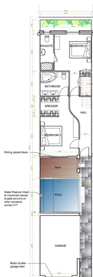
TYPICAL GROUND FLOOR PLAN
