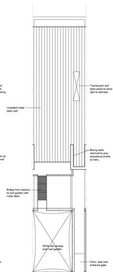
TYPICAL ROOF PLAN
