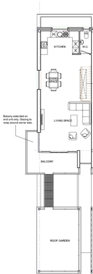
Unit 1. First FLOOR PLAN
